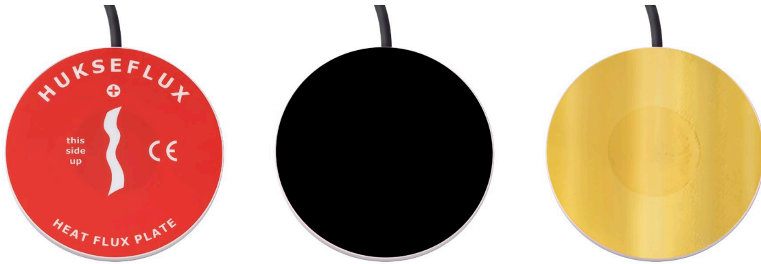
Figure 9.4.1 HFP01 heat flux sensor: with BLK-80 and GLD-80 stickers.
